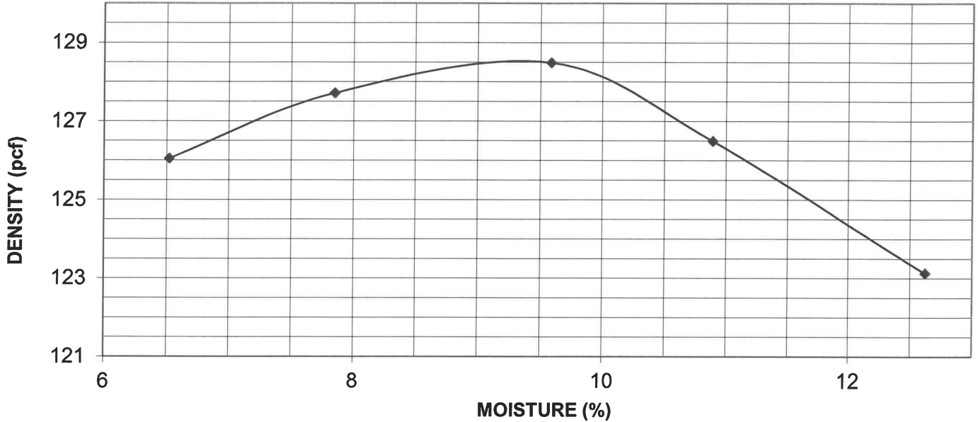
Moisture Content Versus Density
