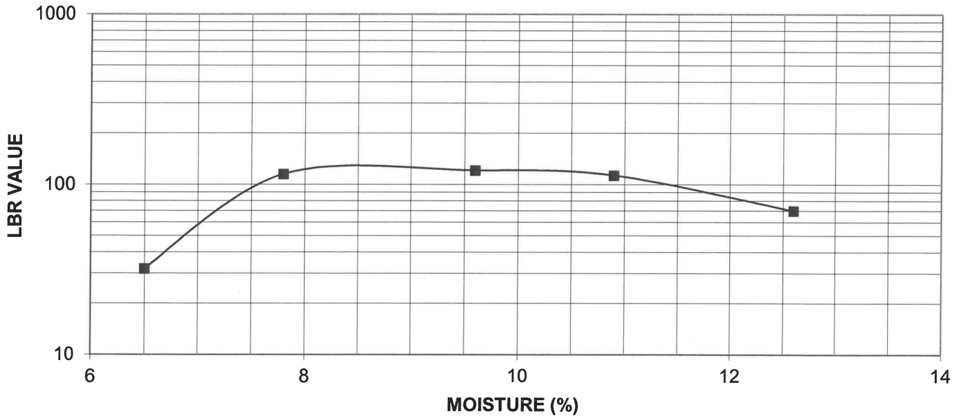
Moisture Content Versus LBR Value
